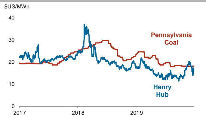
34 US Coal and Natural Gas Power Generation Cost Converted to a $/MWh Equivalent
