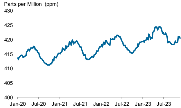
8 Trends in Atmospheric CO 2 Mauna Loa Weekly Average: January 2020 to Present
