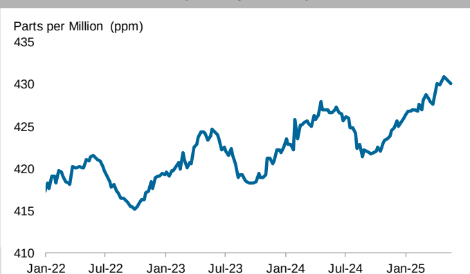
8 Trends in Atmospheric CO 2 Mauna Loa Weekly Average; January 2022 to Present
